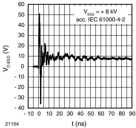
Figure 8. Typical Clamping Performance on + 8 kV - ESD Events (acc. IEC 61000-4-2)
