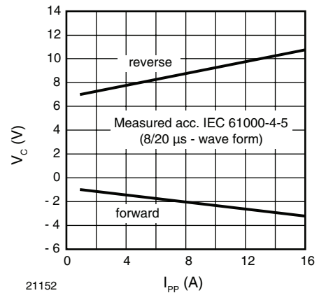
Figure 6. Typical Clamping Voltage vs. Peak Pulse Current I_{PP}
